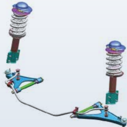
McPherson Strut
